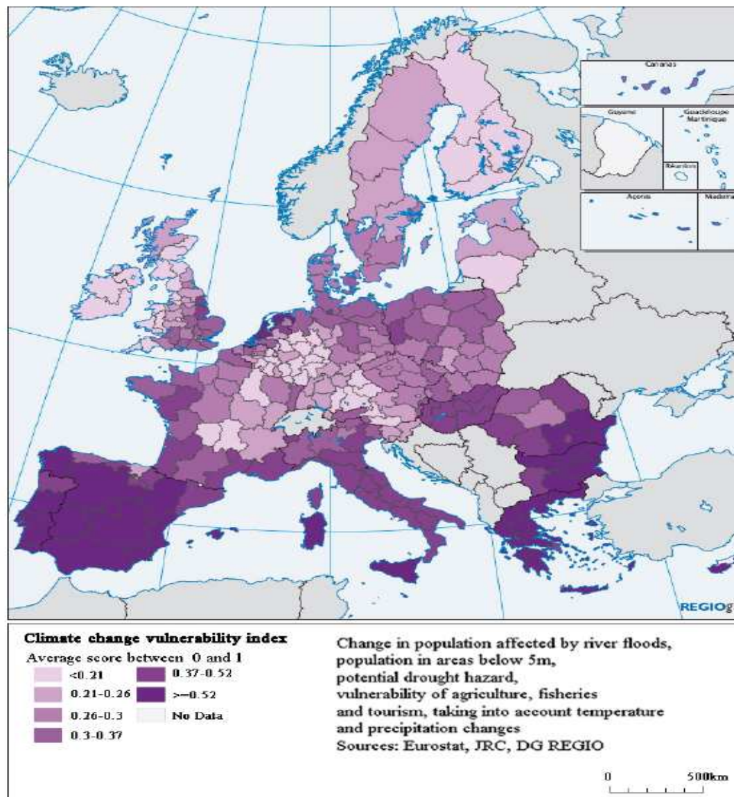
Figure 2. Climate-change vulnerability index
